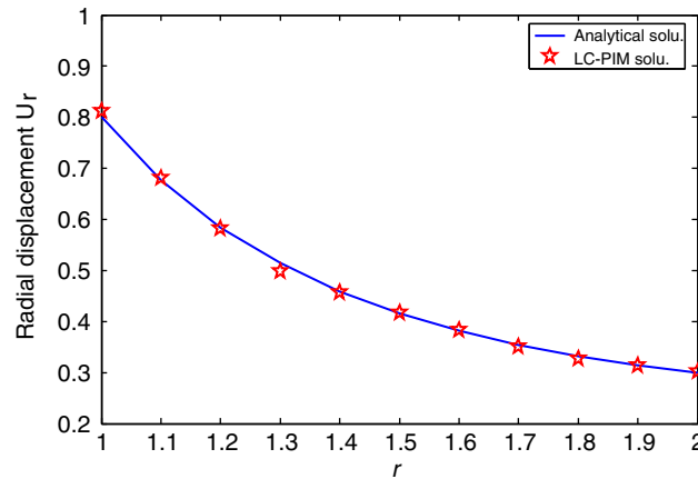
Figure 8. Distribution of the radial displacement along the x -axis for the 3-D Lamé problem.
